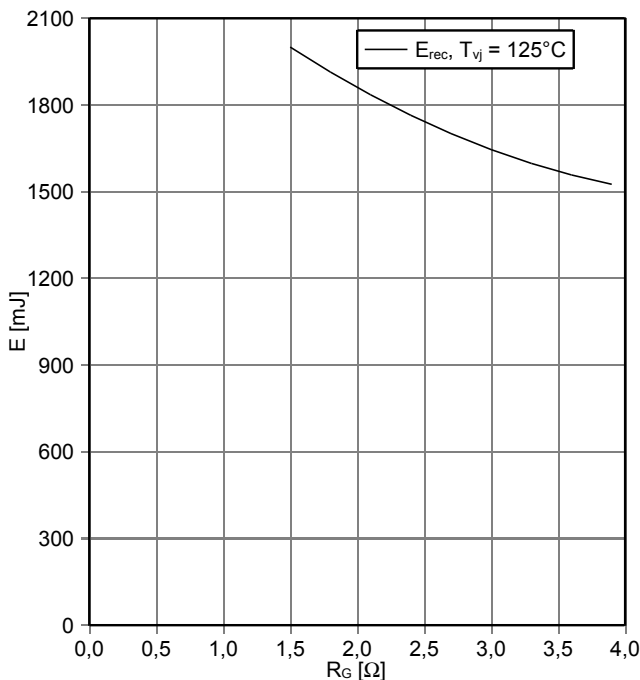
Schaltverluste Diode, Revers (typisch) switching losses Diode, Reverse (typical) E_{rec} = f(R_G) I_F = 500 A, V_{CE} = 3600 V
