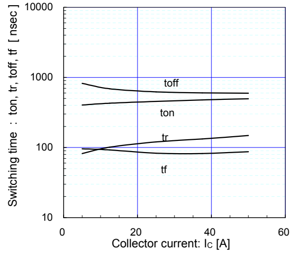
[ Inverter ] a
